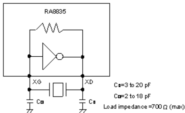
Figure 7-4: Crystal Oscillator
